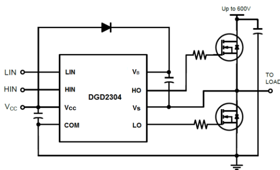
Typical Configuration
