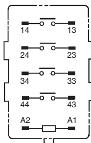
G7J-4A-P(B)(T)
