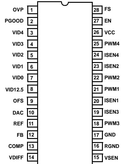
28 LEAD SOIC TOP VIEW
