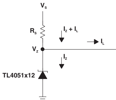
Figure 4. Shunt Regulator
