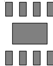
(b) Copper Area = 10mm 2 , \theta_{JA} = 64°C/W
