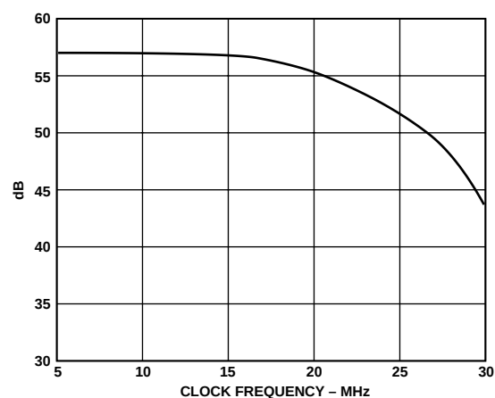
Figure 7. SINAD vs. CLK Frequency (AIN = -0.5 dB)
