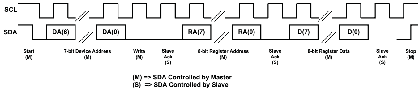
Figure 18. I2C Write
