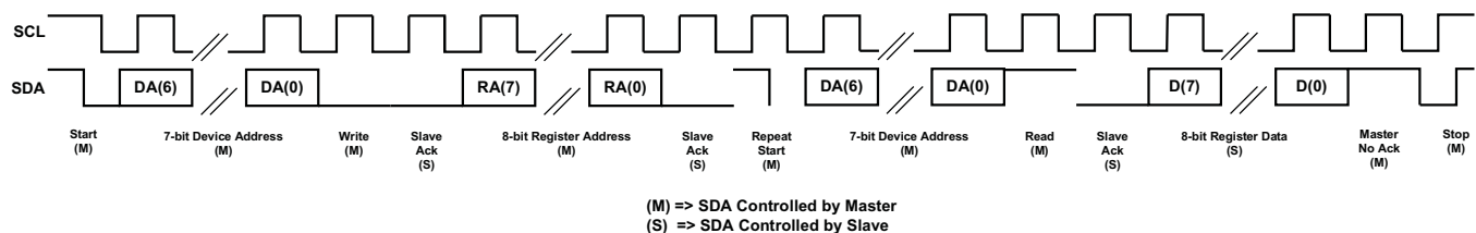
Figure 19. I2C Read
