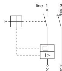
with polarized auxiliary contact -S5
