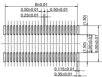
Recommended metal mask pattern Metal mask thickness: When 150 μm (Opening area ratio: 69%)
