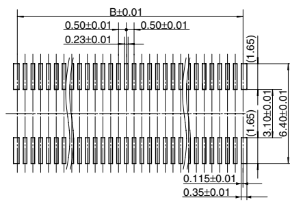
Recommended metal mask pattern Metal mask thickness: When 120 μm (Opening area ratio: 76%)
