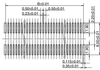
Recommended metal mask pattern Metal mask thickness: When 120 μm (Opening area ratio: 87%)
