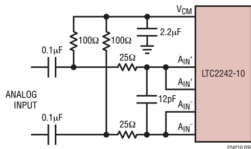
Figure 5. Capacitively-Coupled Drive
