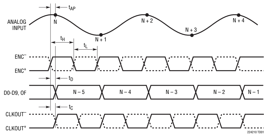
LVDS Output Mode Timing All Outputs Are Differential and Have LVDS Levels
