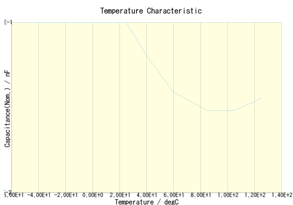
C1608C0G2A101J080AA(DC Bias = 0V) C1608C0G2A101J080AA(DC Bias = 50V)
