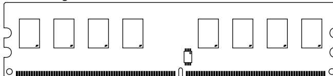
Figure 1: 240-Pin UDIMM (MO-237 R/C E)
