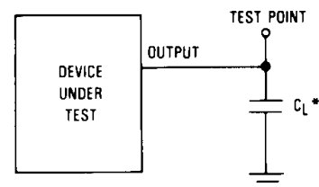
Figure 2. Test Circuit
