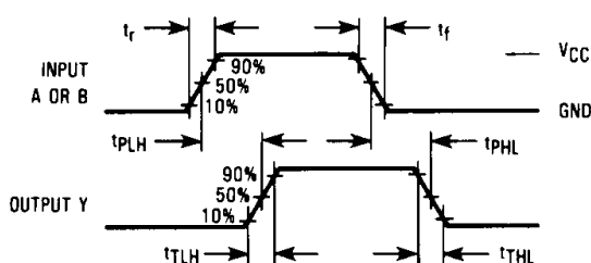
Figure 1. Switching Waveforms
