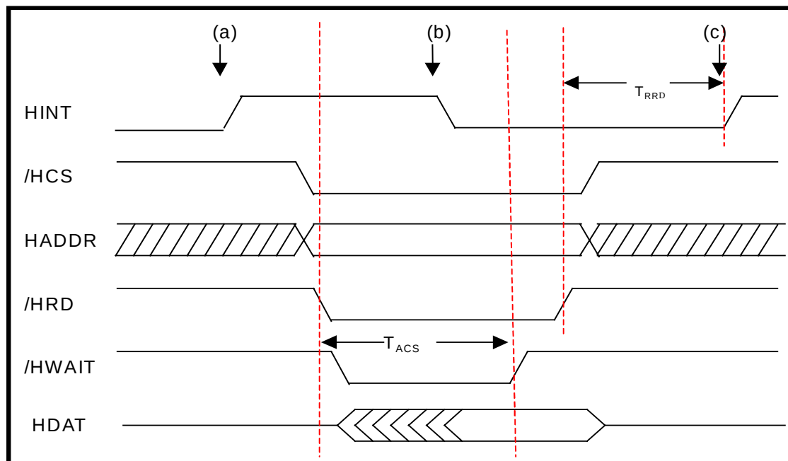
Fig. 7 Interrupt Operation
