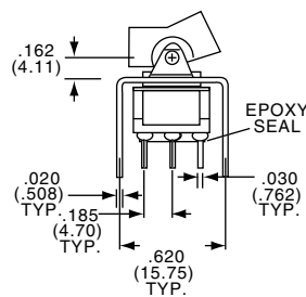
Vertical Support Bracket Single Pole
