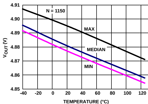
FIGURE 29. V_{OUT} HIGH vs TEMPERATURE, V_+ , V_- = \pm 2.5V , R_L = 1k
