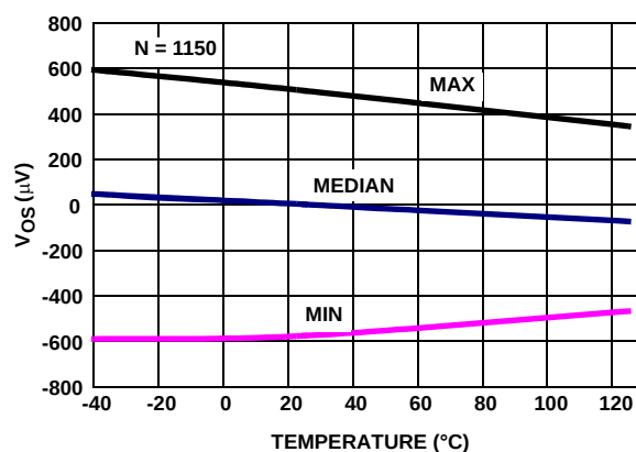
FIGURE 18. V_{OS} vs TEMPERATURE, V_{IN} = 0V , V_+ , V_- = \pm 2.5V
