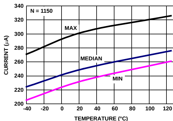
FIGURE 16. ISL28486 SUPPLY CURRENT vs TEMPERATURE, V_+ , V_- = \pm 2.5V ENABLED, R_L = \text{INF}
