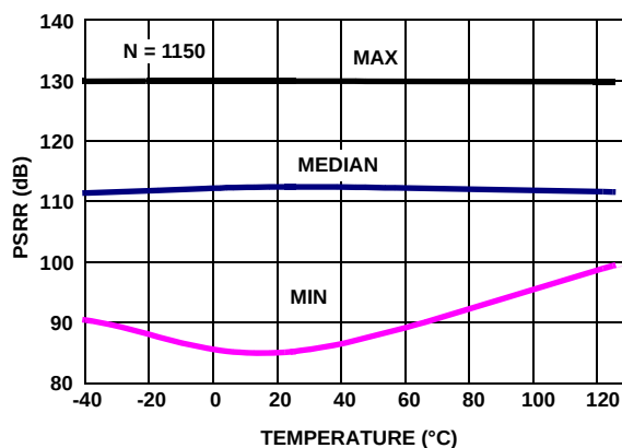
FIGURE 28. PSRR vs TEMPERATURE, V_+ , V_- = \pm 1.2V TO \pm 2.75V
