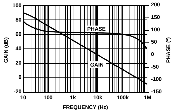
FIGURE 4. A_{VOL} vs FREQUENCY @ 1\text{k}\Omega LOAD
