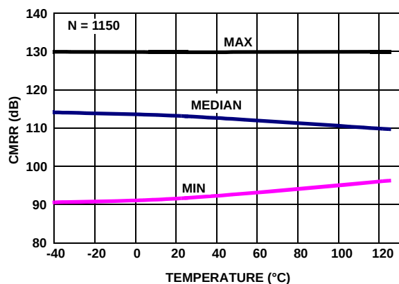
FIGURE 27. CMRR vs TEMPERATURE, V_{CM} = +2.5V TO -2.5V , V_+ , V_- = \pm 2.5V
