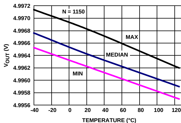
FIGURE 30. V_{OUT} HIGH vs TEMPERATURE, V_+ , V_- = \pm 2.5V , R_L = 100k
