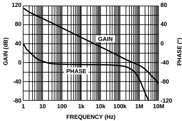
FIGURE 3. A_{VOL} vs FREQUENCY @ 100\text{k}\Omega LOAD
