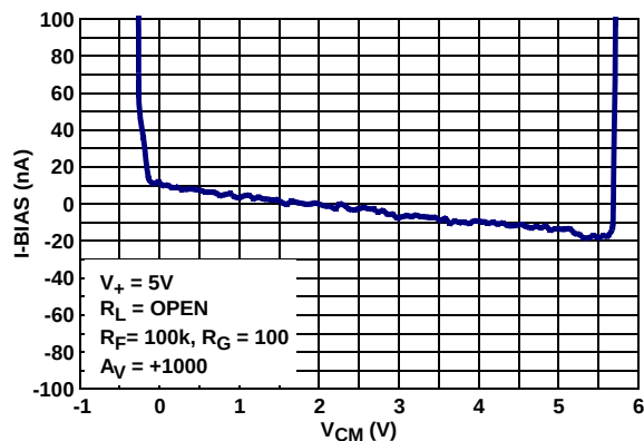
FIGURE 14. INPUT OFFSET CURRENT vs COMMON-MODE INPUT VOLTAGE
