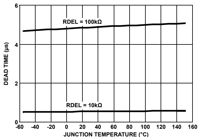
FIGURE 19. DEAD TIME
