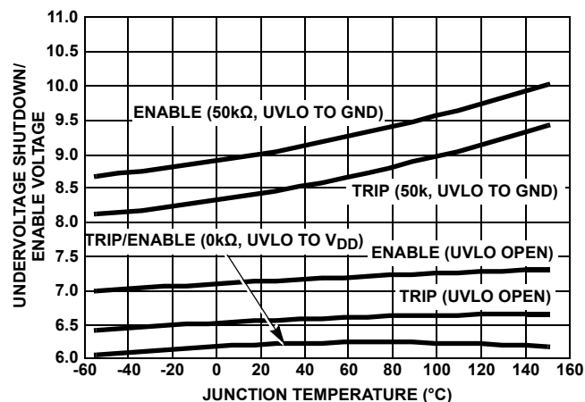
FIGURE 20. UNDERVOLTAGE THRESHOLD
