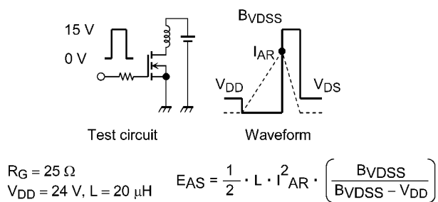
Fig. 8.16 Test Circuit/Waveform
