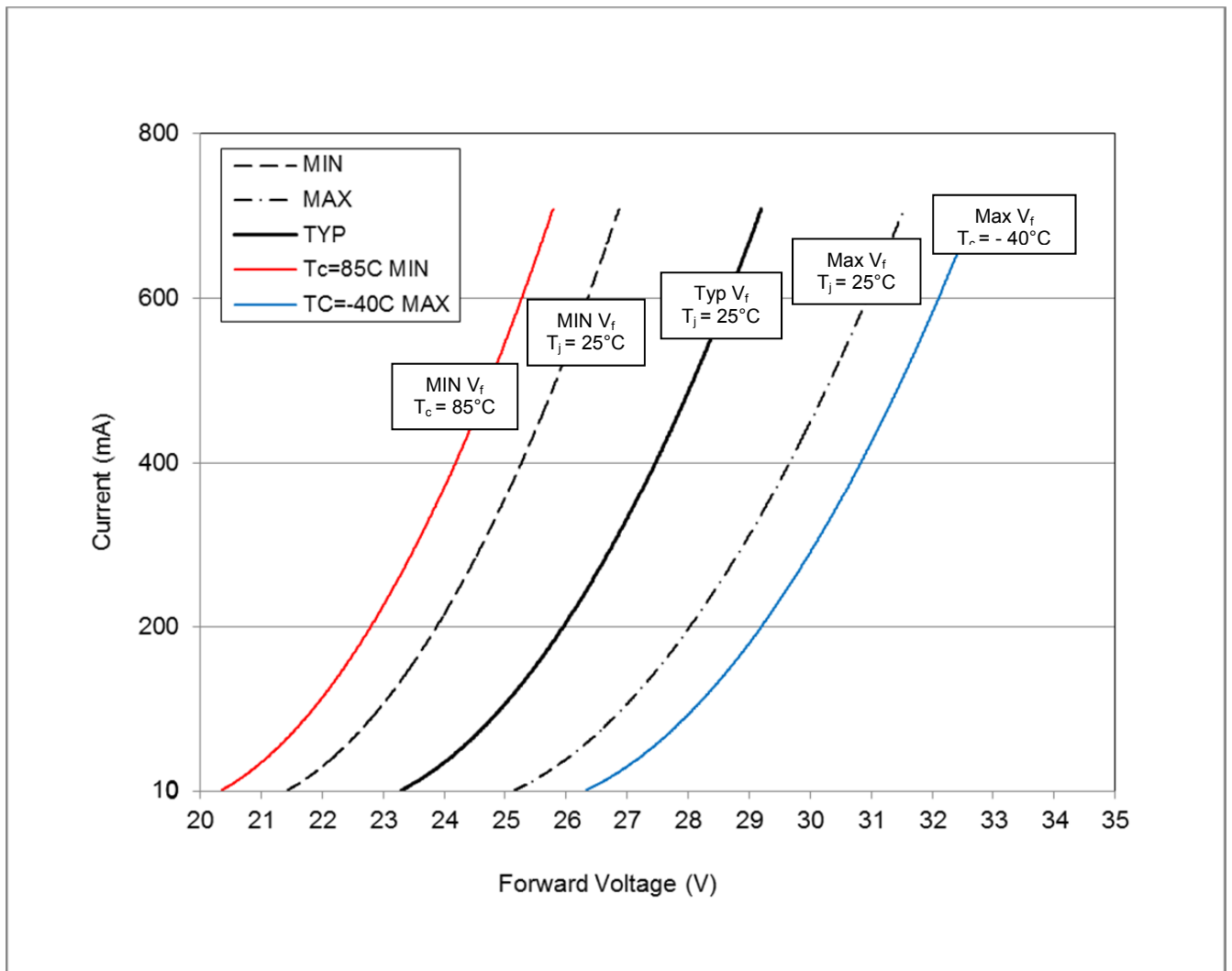
Figure 1: Electrical Characteristics
