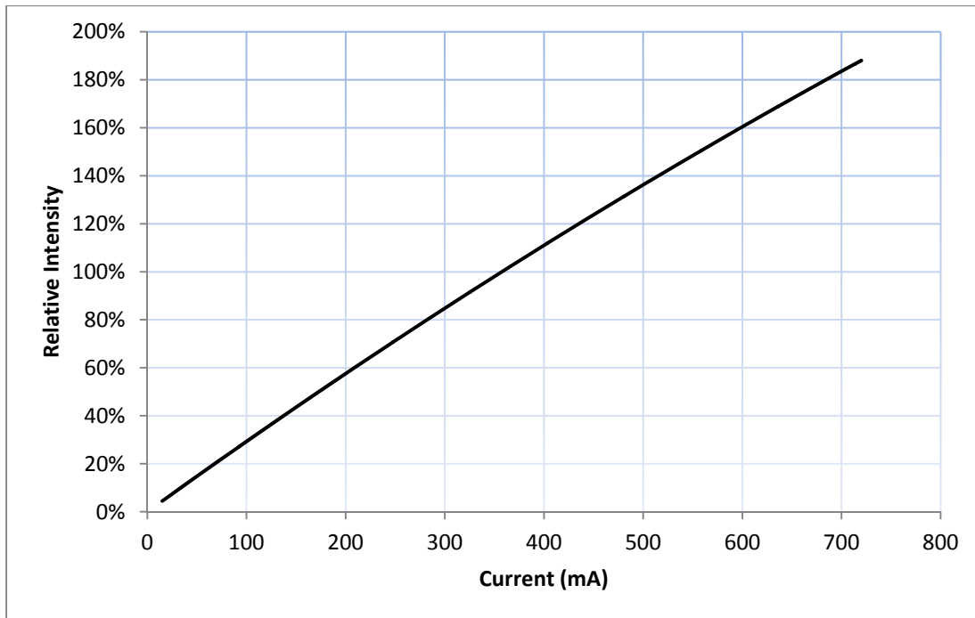
Figure 2: Typical Flux vs. Current, T_j = 25^{\circ}\text{C}
