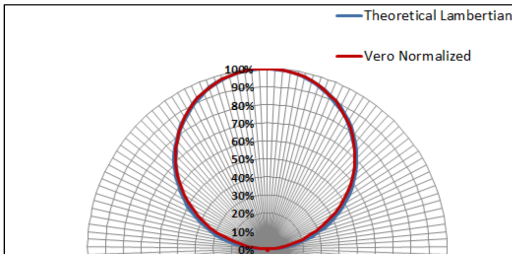
Figure 7: Typical Polar Radiation Pattern
