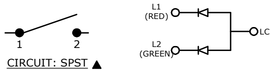
LED SCHEMATIC ▲
