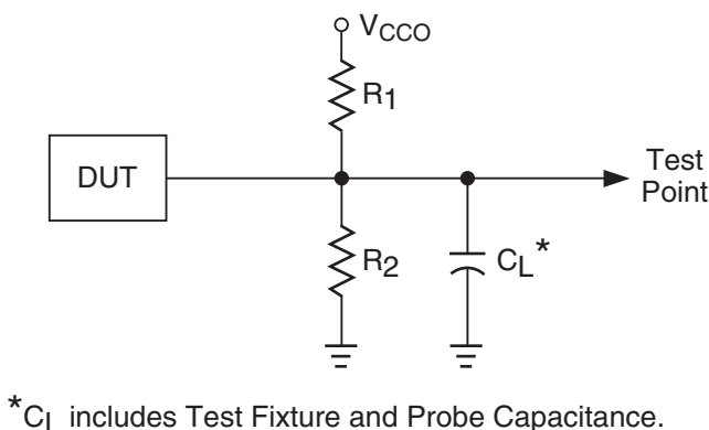
Figure 9. Output Test Load, LVTTTL and LVCMOS Standards
