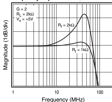
Frequency Response vs. R_f
