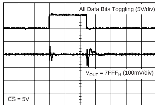
DIGITAL FEEDTHROUGH
