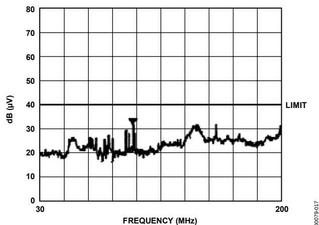
Figure 22. Radiated Emissions
