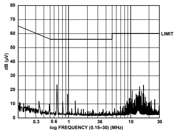
Figure 29. Conducted Emissions
