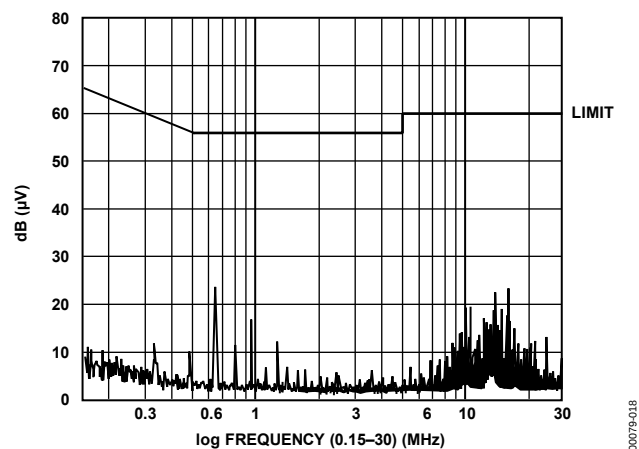
Figure 23. Conducted Emissions
