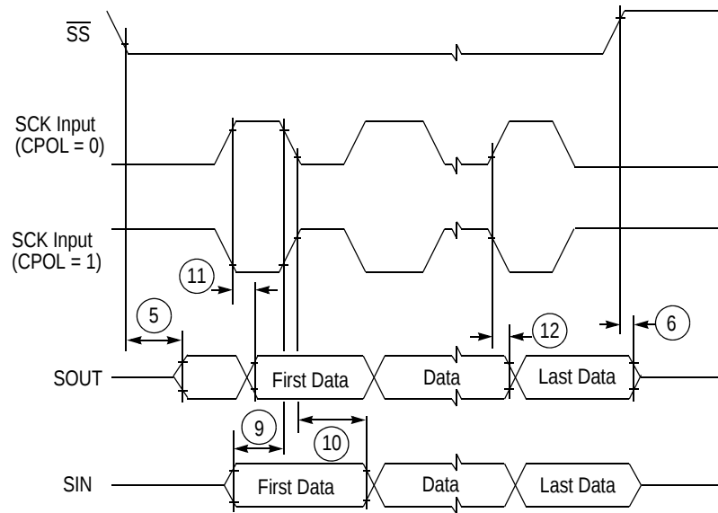
Figure 17. DSPI classic SPI timing — Slave, CPHA = 1
