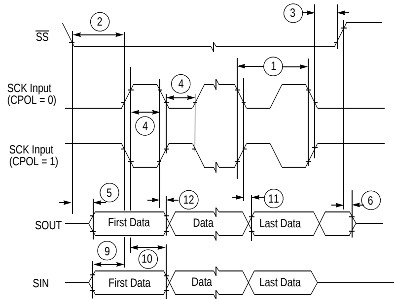
Figure 16. DSPI classic SPI timing — Slave, CPHA = 0
