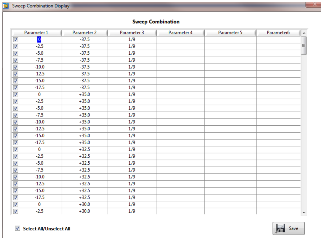
Figure 14. TLK10232 EVM GUI High-Speed Link Optimizer Setup
