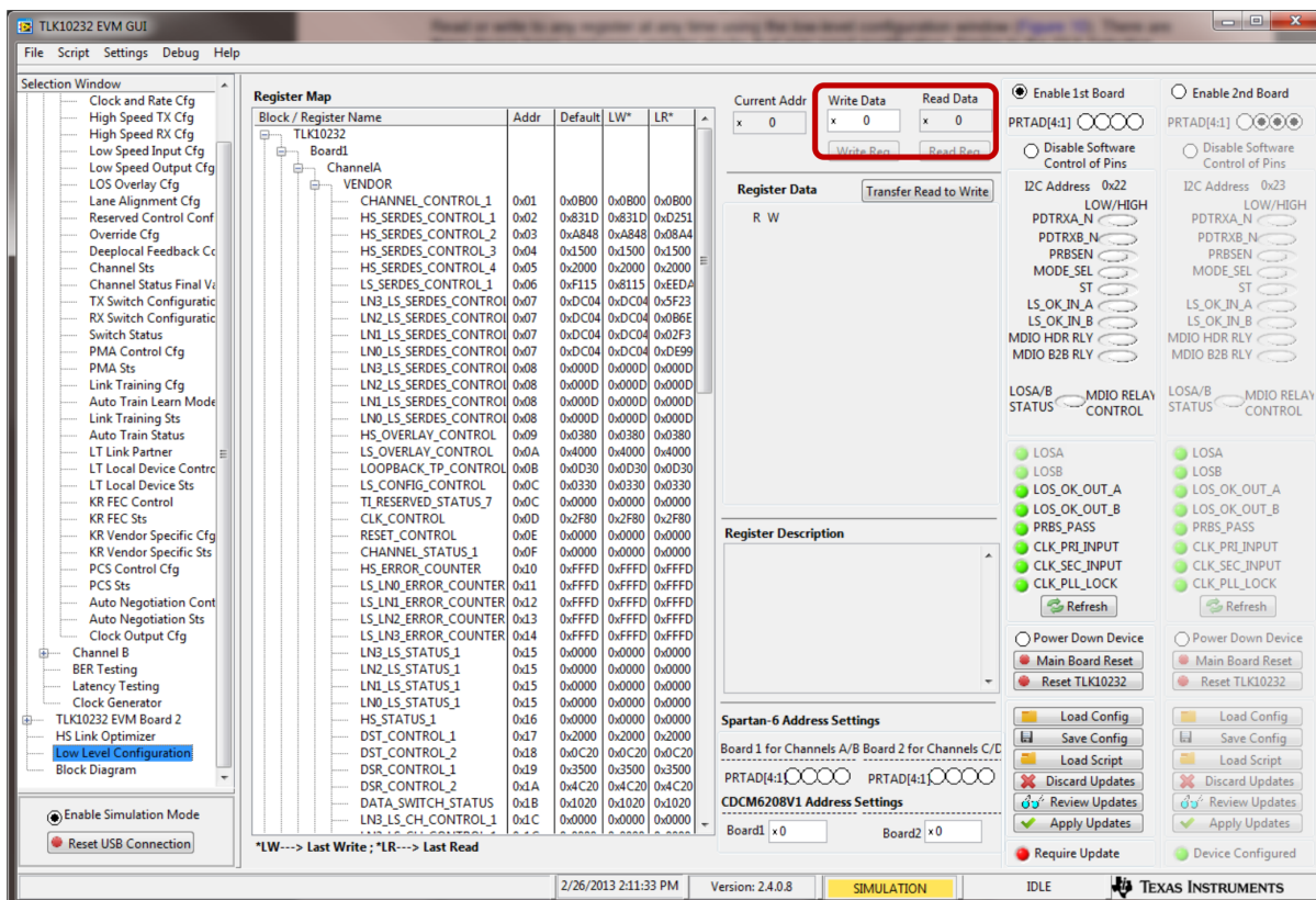
Figure 10. TLK10232 EVM GUI Low-Level Device Configuration
