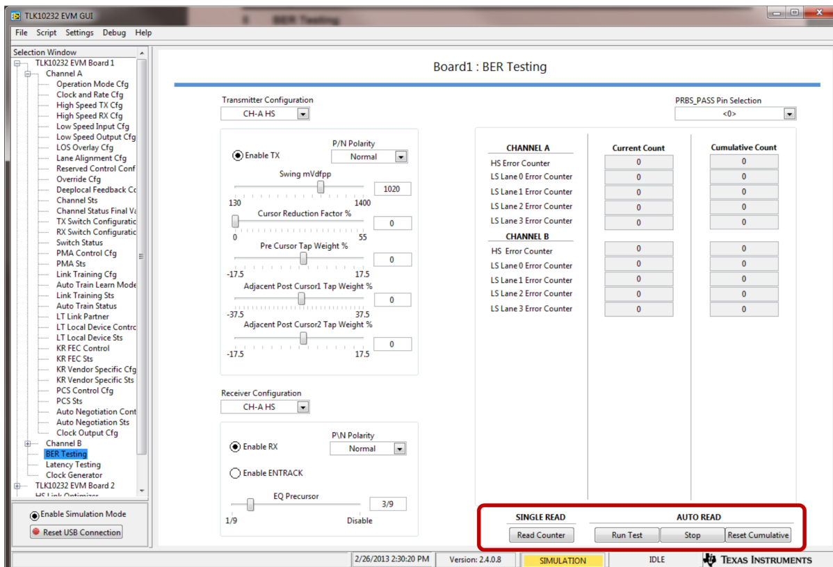
Figure 11. TLK10232 EVM GUI High-Level BER Testing
