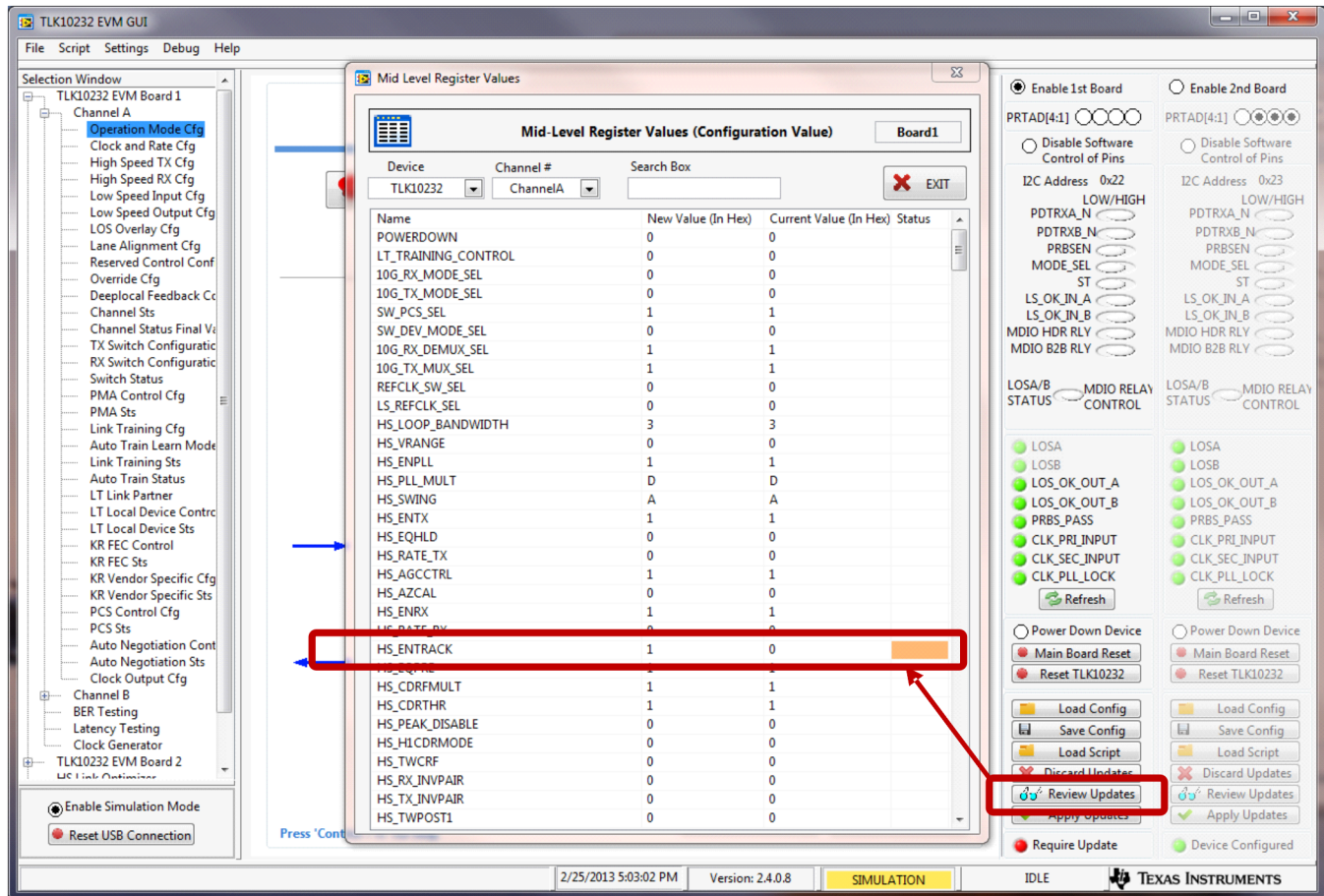
Figure 5. TLK10232 EVM GUI High-Level Review Updates
