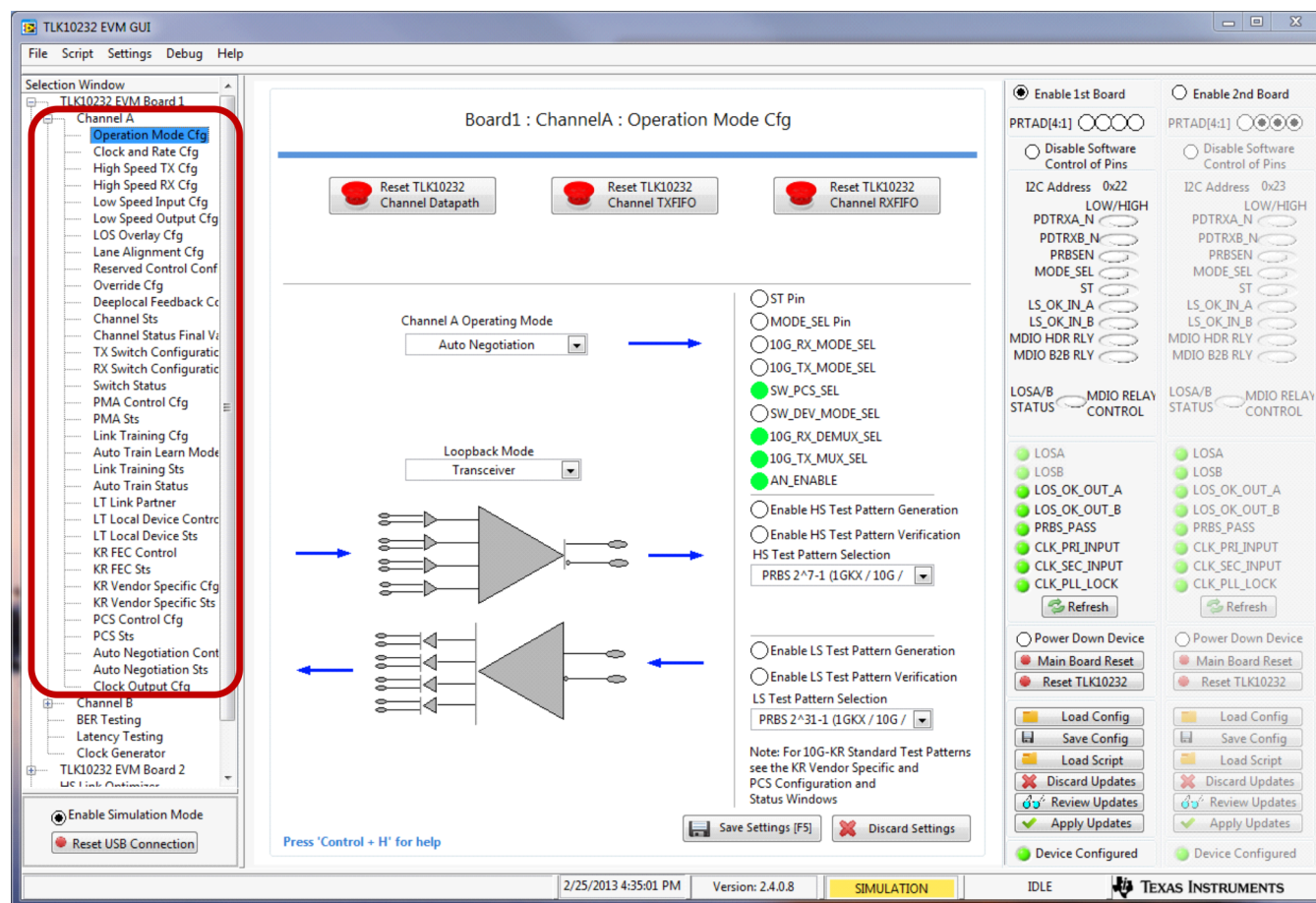
Figure 2. TLK10232 EVM GUI Hierarchical Selection Window Tree
