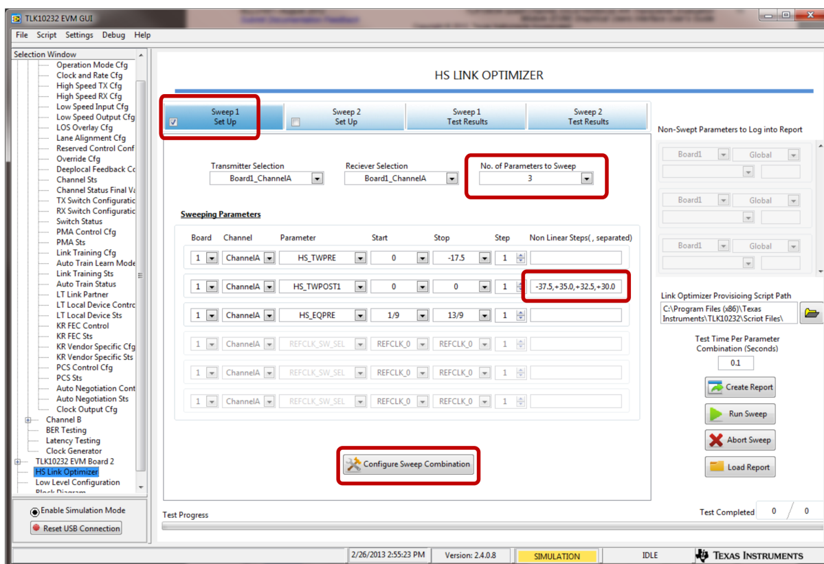
Figure 13. TLK10232 EVM GUI High-Speed Link Optimizer Setup
