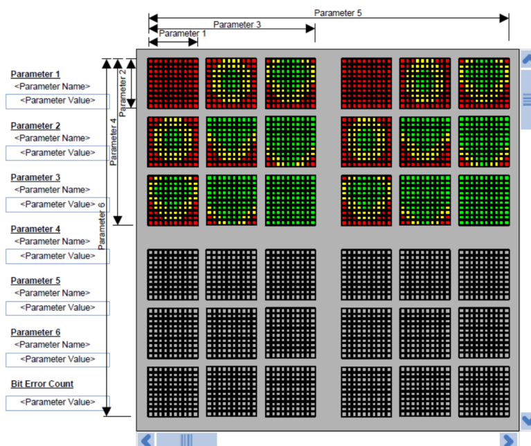
Figure 16. TLK10232 EVM GUI High-Speed Link Optimizer Sweep Results Matrix
