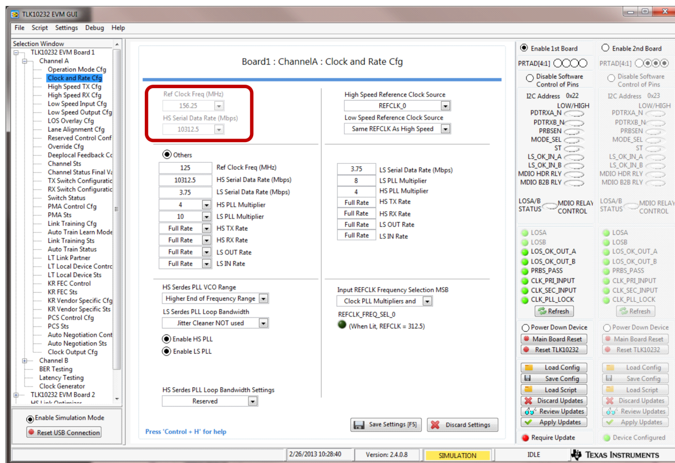
Figure 6. TLK10232 EVM GUI High-Level Device Clock and Rate Configuration
