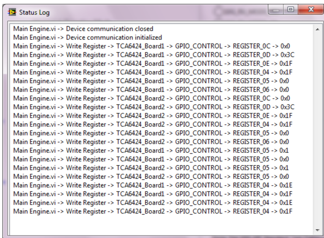
Figure 23. TLK10232 EVM GUI Status Log Window
