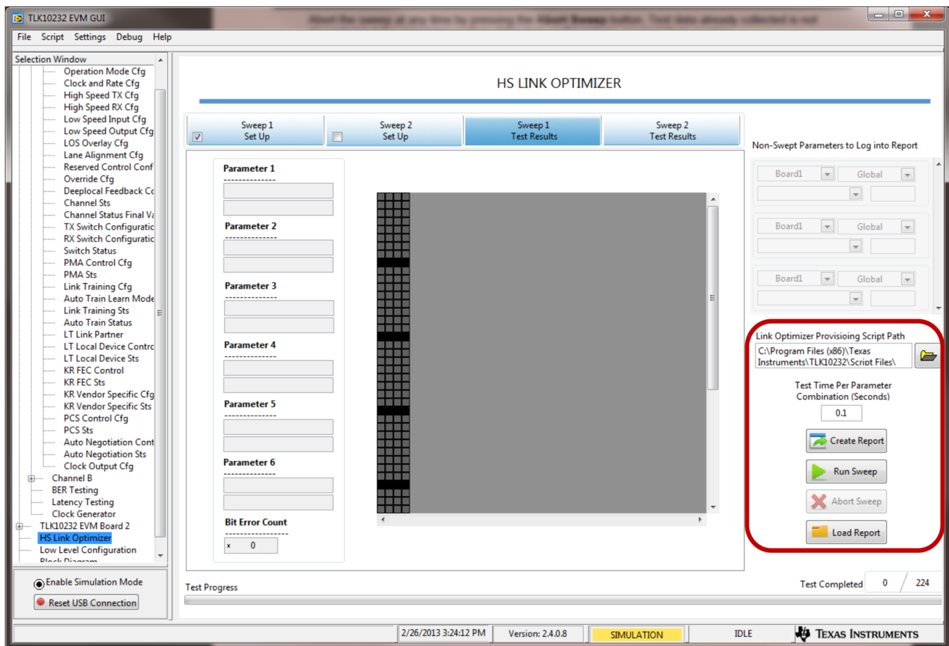
Figure 17. TLK10232 EVM GUI High-Speed Link Optimizer Test Control Buttons
