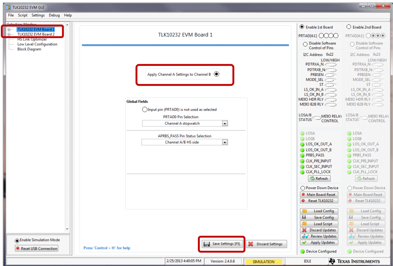
Figure 1. TLK10232 EVM GUI Board 1 Window
