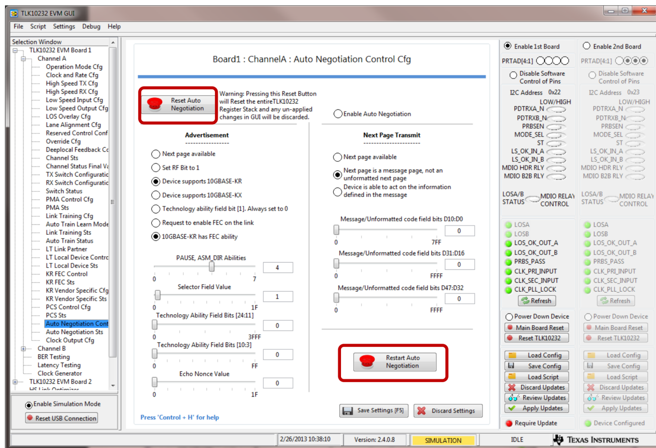
Figure 8. TLK10232 EVM GUI High-Level Device Immediate Action Pushbuttons
