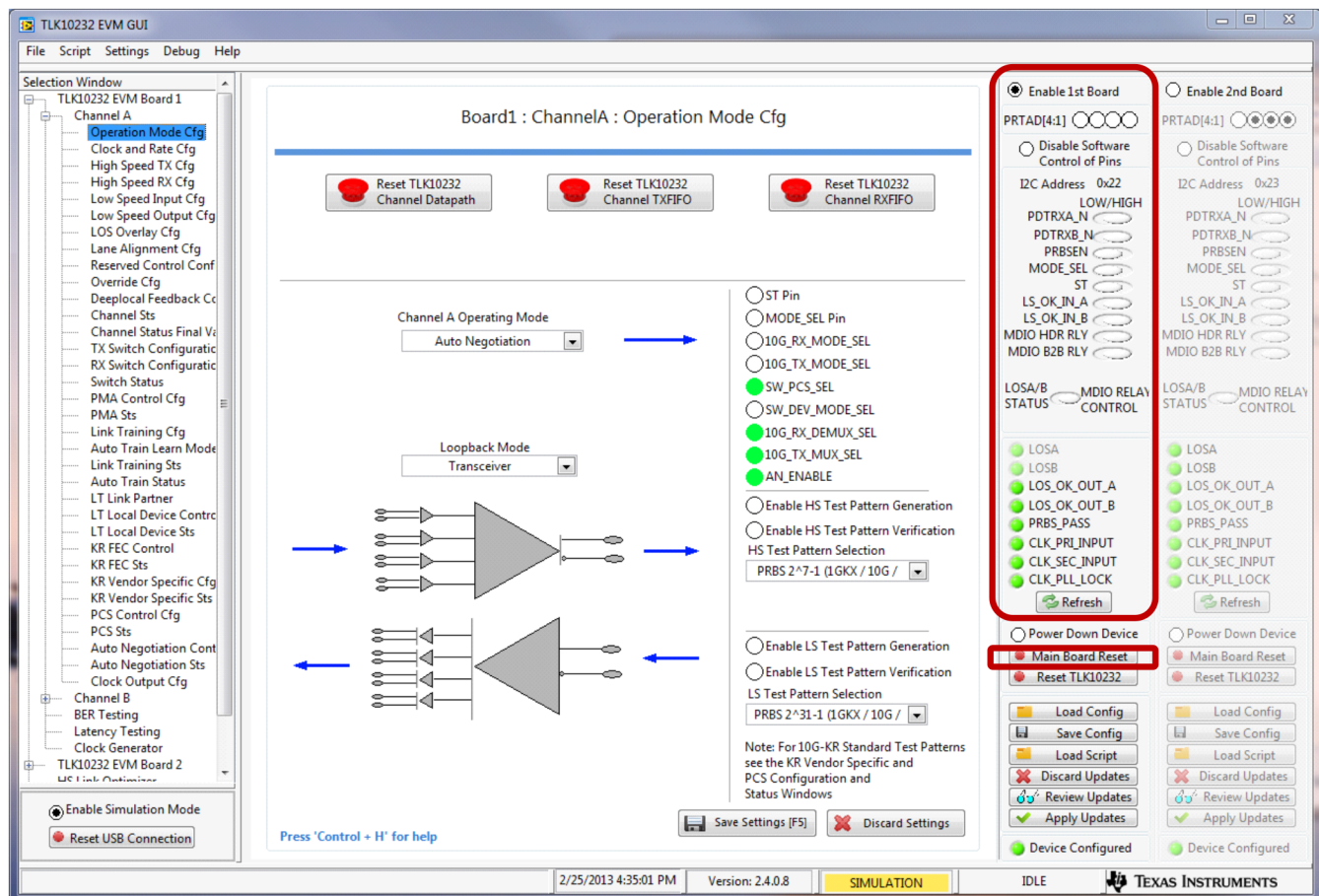
Figure 3. TLK10232 EVM GUI Software Control of TLK10232 I/O Pins and Main Reset
