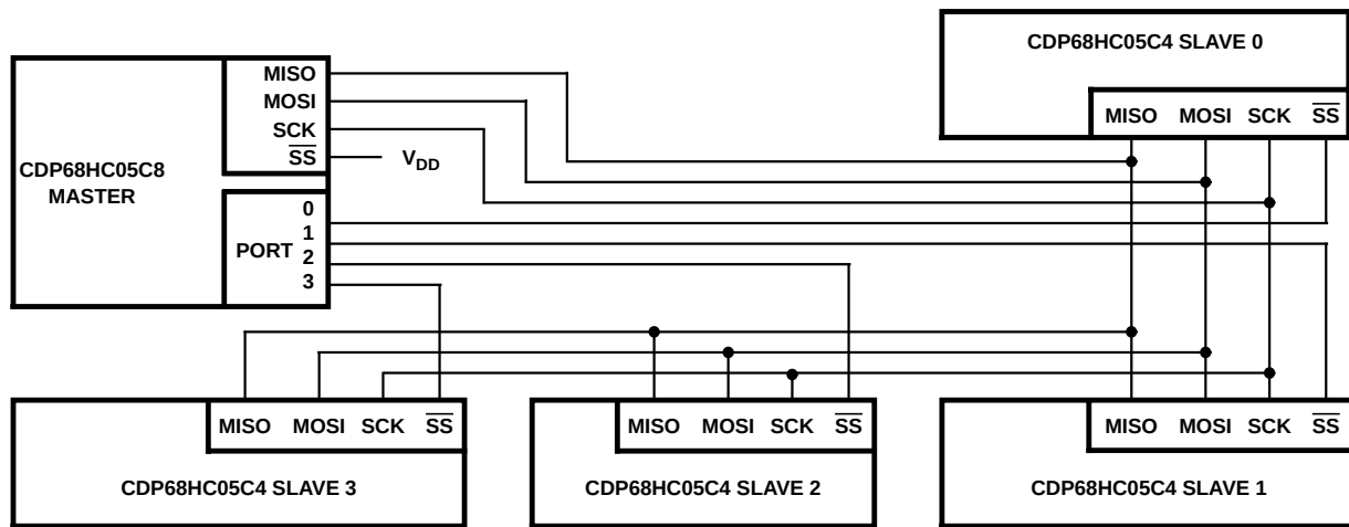
FIGURE 27. MASTER-SLAVE SYSTEM CONFIGURATION (SINGLE MASTER, FOUR SLAVES)
