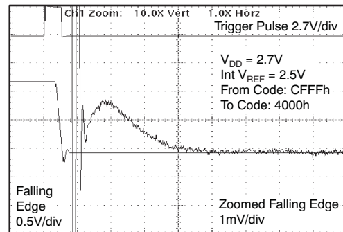
Figure 54. Full-Scale Settling Time: 2.7-V Falling Edge
