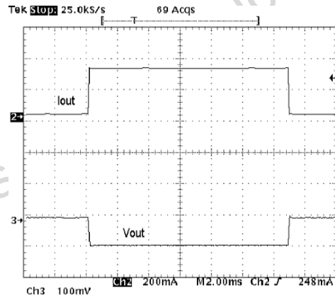
Figure 10 : Load Transient
