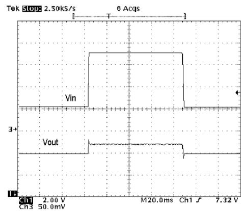
Figure 9 : Line Transient
