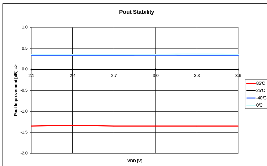
Figure 76: Pout Stability
