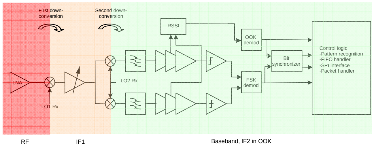
Figure 14: Receiver Architecture
