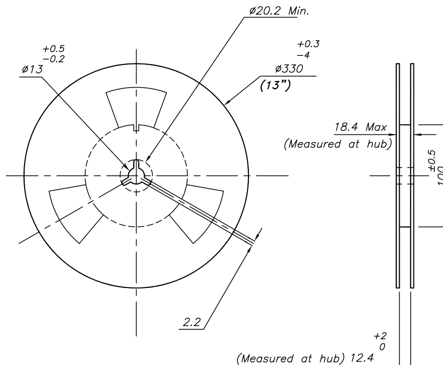
Figure 67. Reel outline
