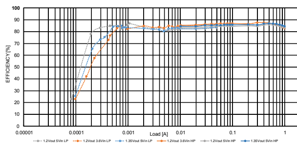
Figure 4. BUCK2 efficiency
