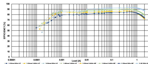
Figure 6. BUCK4 efficiency
