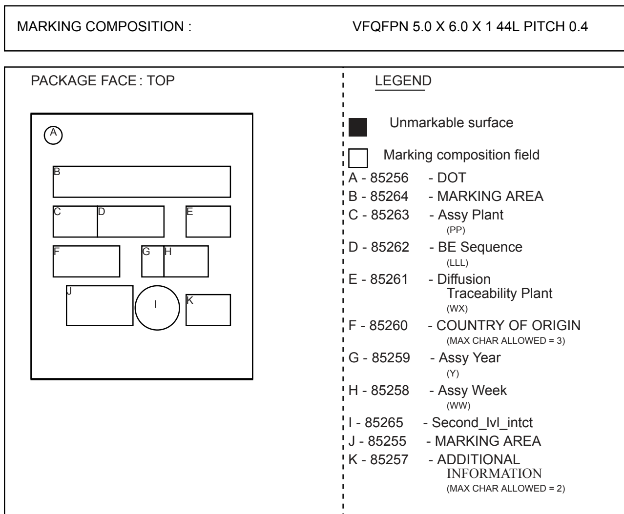
Figure 68. Marking composition
