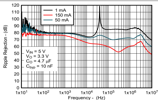
Figure 5-20. Ripple Rejection vs Frequency (New Chip)
