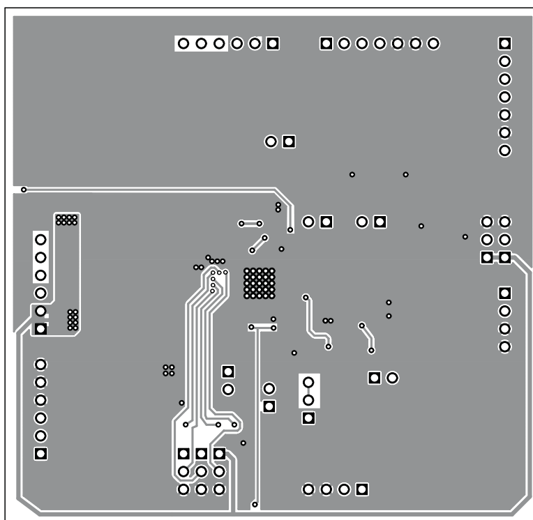
Figure 4. Bottom Layer
