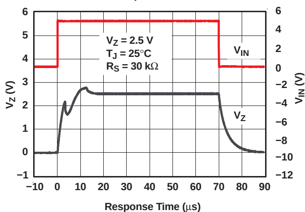
Figure 6. Start-Up Characteristics
