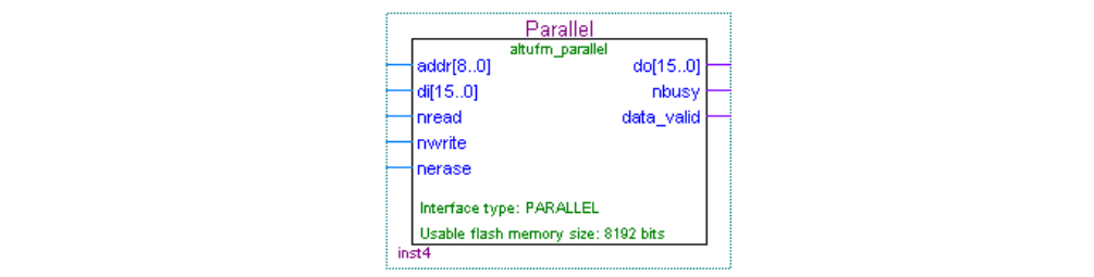
Figure 9-41. altufm Megafunction Symbol for Parallel Interface Instantiation
