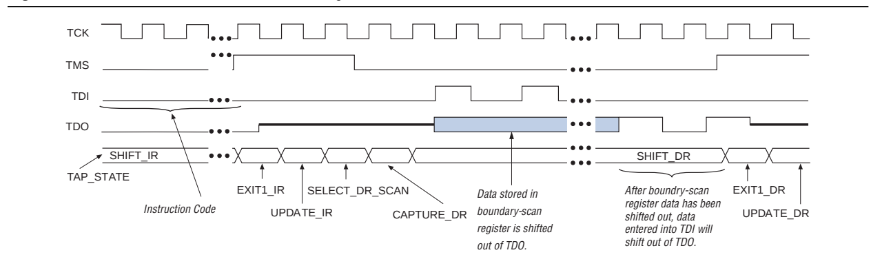
Figure 13–9. SAMPLE/PRELOAD Shift Data Register Waveforms
