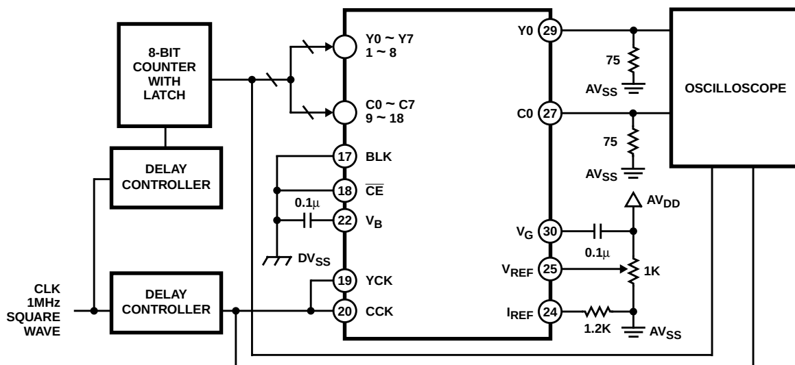
FIGURE 3. SETUP HOLD TIME AND GLITCH ENERGY
