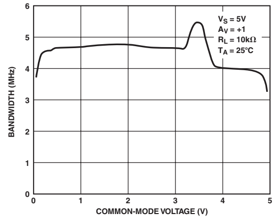
TPC 23. Frequency vs. Common-Mode Voltage ( V_S = 5.0\text{ V} )
