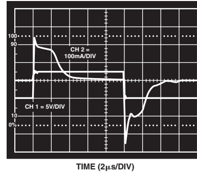
Figure 6. Scope Photo of the V_{\text{COM}} Instantaneous Peak Current
