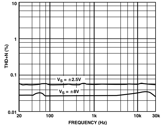
Figure 4. THD+N vs. Frequency Graph
