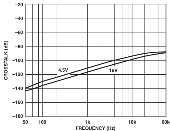
TPC 21. Channel A vs. Channel B Crosstalk
