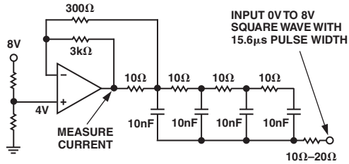
Figure 5. V_{\text{COM}} Test Circuit with Supply Voltage at 16 V
