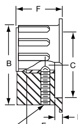
(2) 6-32 SET SCREWS
