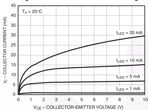
Fig. 18 Collector Current vs. Collector Voltage
