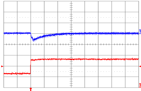
Fig. 1.2V.7: Output voltage response for V_{out} = 1.2 V to positive load current step change from 2.5 A to 5 A with slew rate of 5 \text{ A}/\mu\text{s} at V_{in} = 12 V. Top trace: output voltage (100 mV/div.); Bottom trace: load current (2 A/div.). C_o = 47 \mu\text{F} ceramic. Time scale: 20 \mu\text{s} /div.
