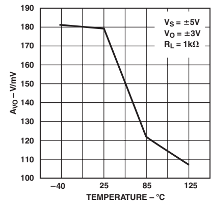
TPC 18. A_{V0} vs. Temperature at \pm 5 V
