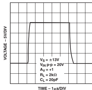
TPC 33. Large Signal Response at G = +1
