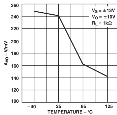
TPC 17. A_{V0} vs. Temperature at \pm 13 V
