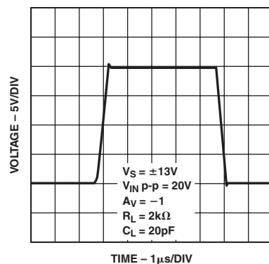
TPC 36. Large Signal Response at G = -1
