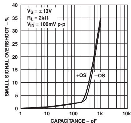
TPC 30. Small Signal Overshoot vs. Load Capacitance
