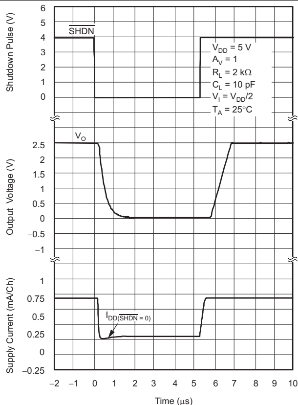
Figure 33. Shutdown Supply Current/output Voltage vs Time
