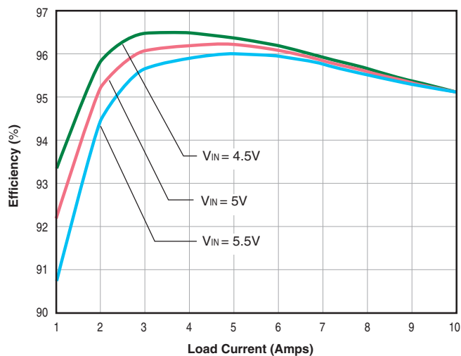
LSN-3.3/10-D5 Efficiency vs. Line Voltage and Load Current
