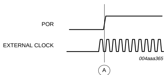
Fig 4. External clock with respect to power-on reset
