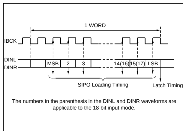
FIGURE 4. SIPO Input Data Loading Timing.
