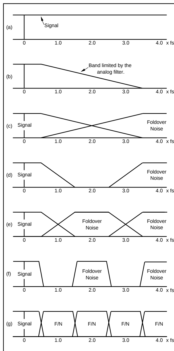
FIGURE 2. The Associated Spectra of the Oversampling-Decimating Technique.
