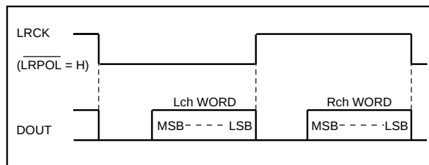
FIGURE 8. Output Timing.
