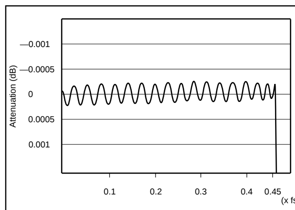
DF1750 1/2 Decimating Passband Frequency Response.
