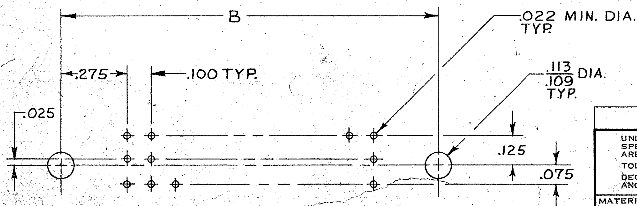
P.C. BOARD LAYOUT
