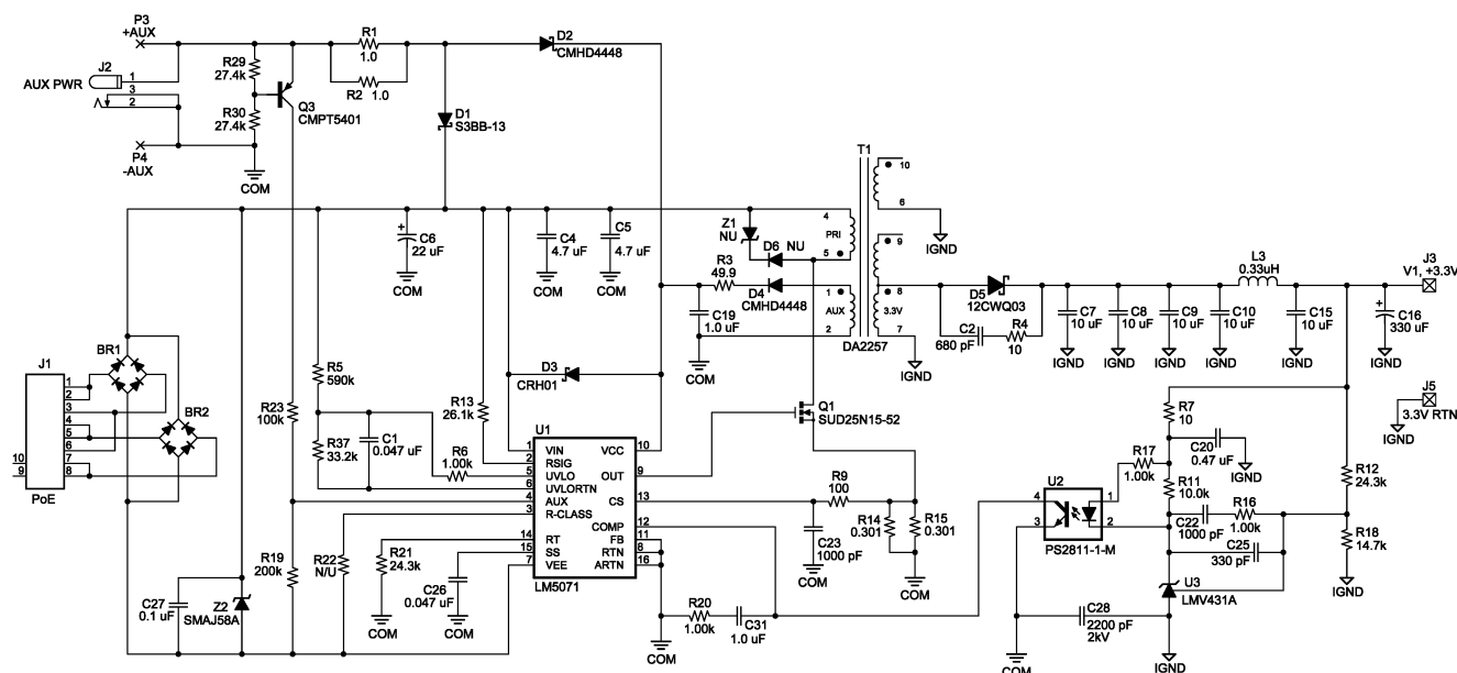
Figure 16. Single Isolated Output with Diode Rectification and 12V Auxiliary Supply
