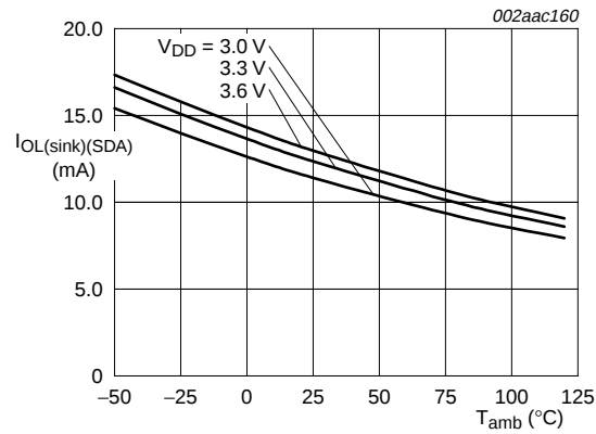
Fig 17. \overline{\text{EVENT}} sink current at 0.6 V versus temperature
