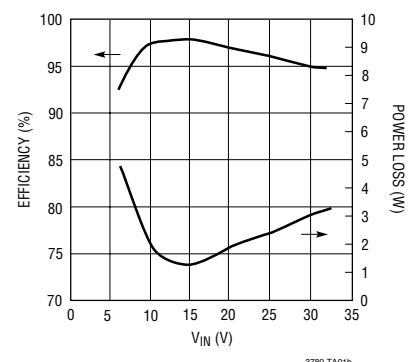
Efficiency and Power Loss V_{OUT} = 12V , I_{LOAD} = 5A
