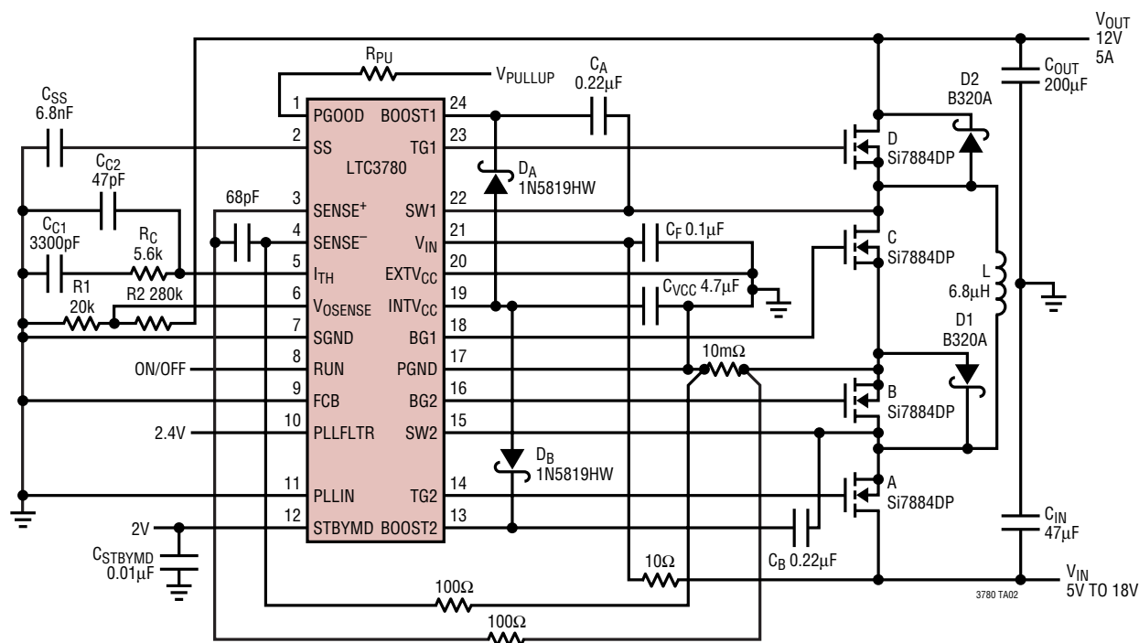
Figure 13. LTC3780 12V/5A, Buck-Boost Regulator
