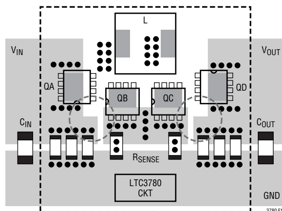
Figure 10. Switches Layout
