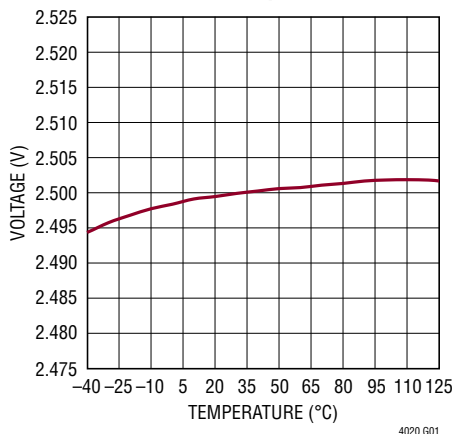
V_{\text{FLOAT(CC/CV)}} or, V_{\text{ABSORB(Lead-Acid)}} Reference vs Temperature
